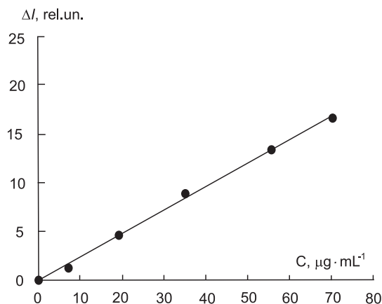
Fig. 2. Dependence of \Delta I on the concentration of L -cystine in the chemiluminescence system H_2L - H_2O_2 - Hb . c(\text{NaOH}) = 0.05 \text{ mol} \cdot \text{L}^{-1} , c(H_2O_2) = 8.5 \cdot 10^{-4} \text{ mol} \cdot \text{L}^{-1} , c(H_2L) = 1 \cdot 10^{-4} \text{ mol} \cdot \text{L}^{-1} , C(Hb) = 5 \cdot 10^{-2} \mu\text{g} \cdot \text{mL}^{-1}
